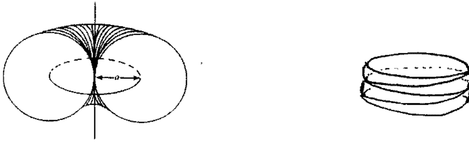
Figure 5: Kepler's 'apple'
