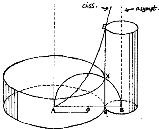
Figure 4: The cissoid revolved about its asymptote has the same volume as the semi-circle revolved about its tangent
