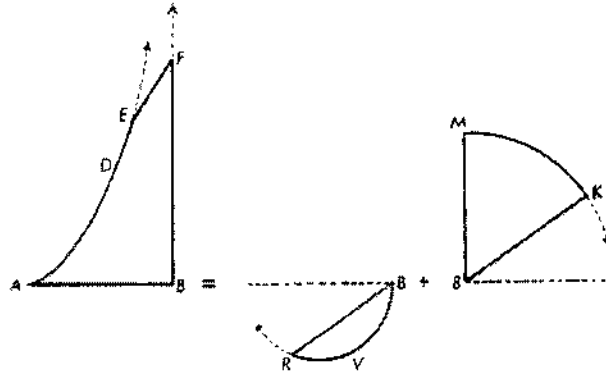
Figure 7: ADEFBA = \text{segment } BVR + \text{sector } BKM
