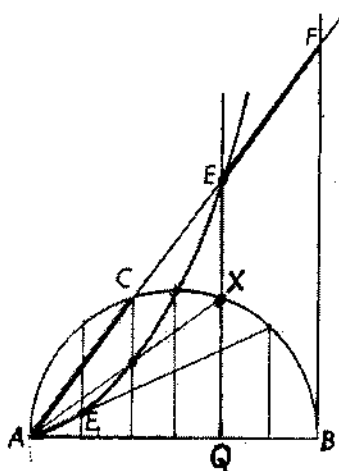
Figure 3: The cissoid of Diocles: the locus of E as C varies subject to arc AX = \text{arc } BC .
