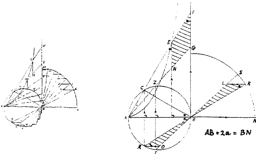
Figure 6: Huygens' diagram (28 May 1658 version, and redrawn)
