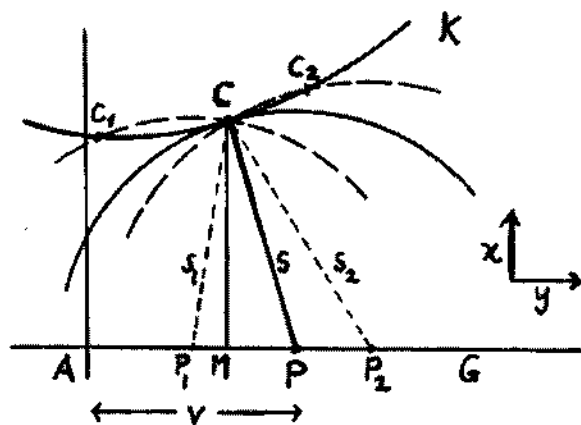
Figure 1: The normal to K through its point C
