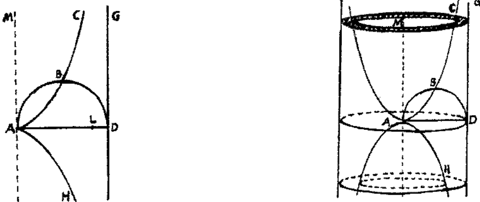
Figure 8: Sluse's infinite glass
